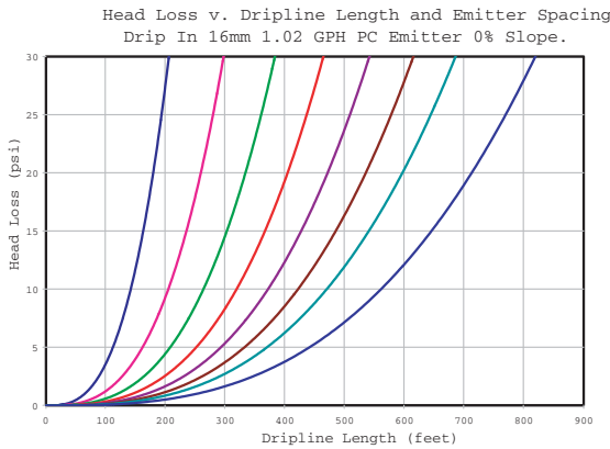
16mm Drip In PC – Maximum Recommended Dripline Length (Feet) (0.550" I.D./0.640" O.D./0.045" Wall)
