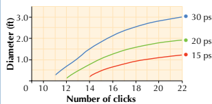
Diameter of Throw 360°
