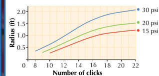
Radius of Throw 180°
