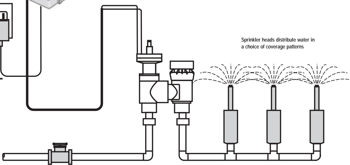
Main shut-off valve shuts off water from supply line
